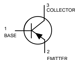
CASE 318-08, STYLE 6 SOT-23 (TO-236AB)
